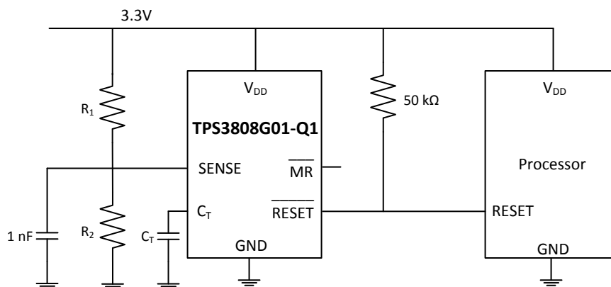
Figure 15. TPS3808G01-Q1 Typical Application
