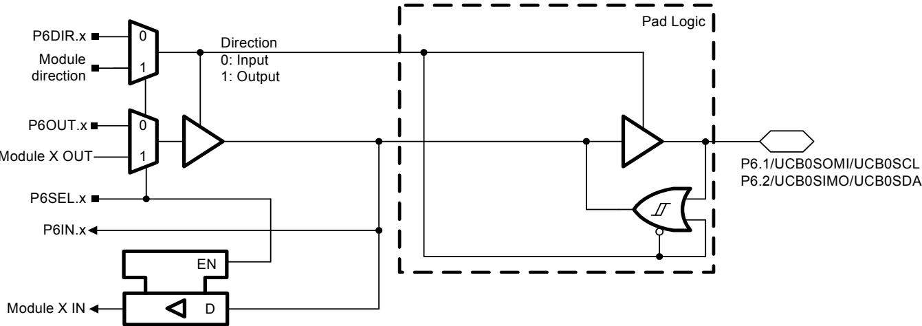
Port P6 (P6.1 and P6.2) pin functions
