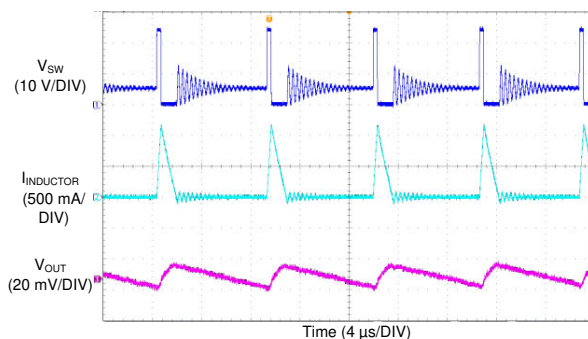
图 8-11. LM76005 Switching Waveform and Output Ripple
