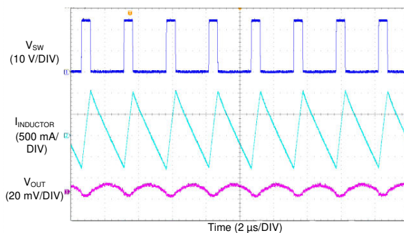
图 8-13. LM76005 Switching Waveform and Output Ripple
