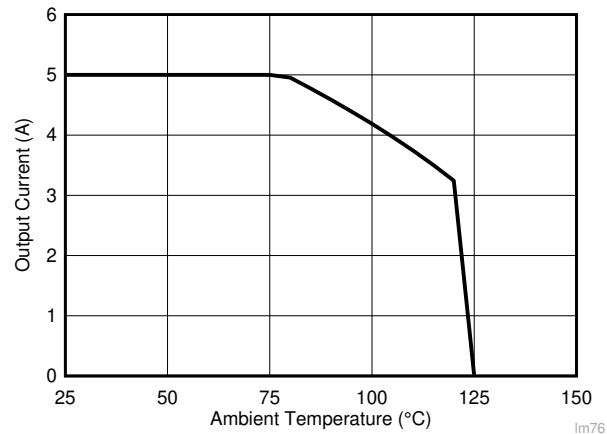
图 8-3. LM76005 Safe Operating Area (5 V OUT , 400 kHz, R_{\theta JA}=18.8\text{ }^{\circ}\text{C/W} )
