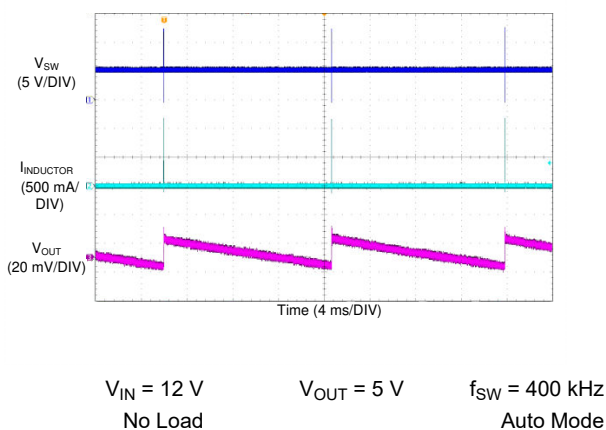
图 8-8. LM76005 Switching Waveform and Output Ripple
