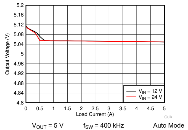
图 8-5. LM76005 Load and Line Regulation
