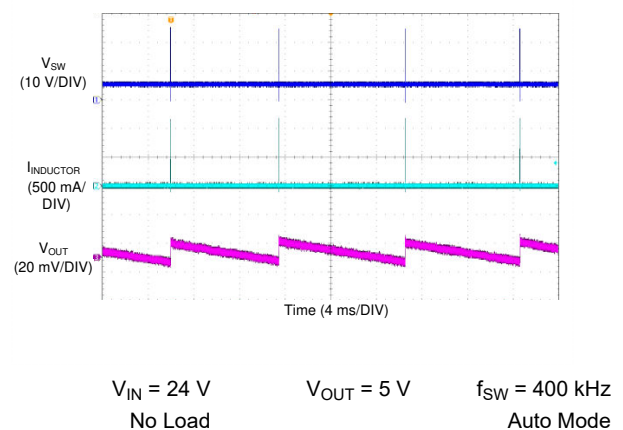
图 8-9. LM76005 Switching Waveform and Output Ripple
