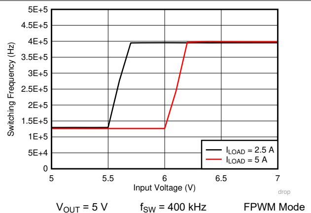
图 8-7. LM76005 Frequency Dropout
