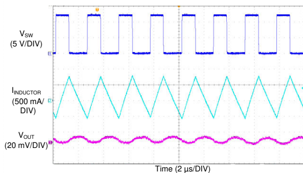
图 8-12. LM76005 Switching Waveform and Output Ripple
