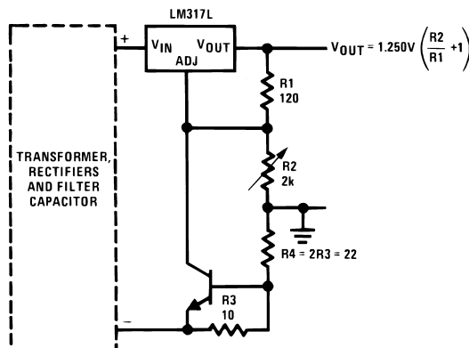
Figure 25. Adjustable Regulator With Current Limiter
