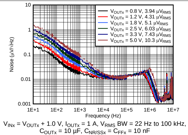
图 10. Noise vs Frequency and Output Voltage
