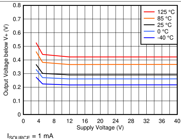
图 23. Output High Voltage vs. Supply Voltage
