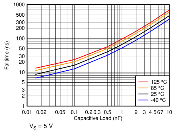
图 54. t_{FALL} vs. Capacitive Load at 5V
