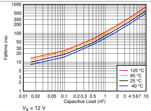
图 56. t_{FALL} vs. Capacitive Load at 12V
