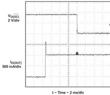
图 9-33. 3- \Omega Load Connected to Enabled Device
