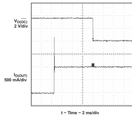
图 9-25. 2- \Omega Load Connected to Enabled Device
