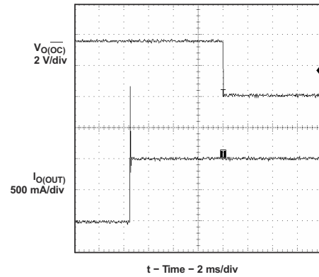
图 9-34. 2- \Omega Load Connected to Enabled Device
