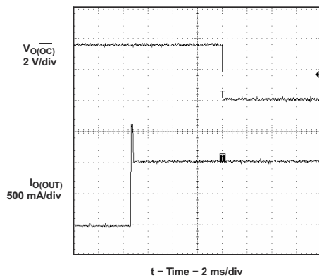
图 9-24. 3- \Omega Load Connected to Enabled Device
