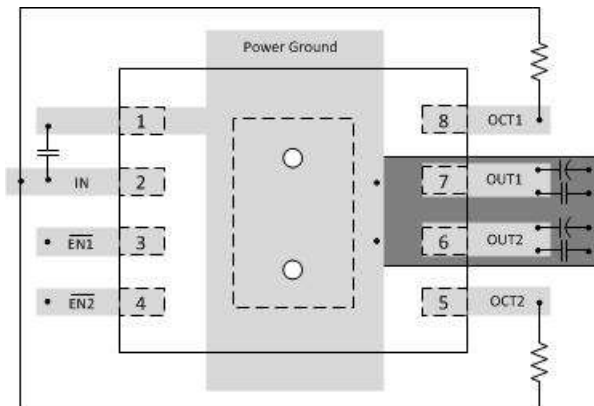
图 11-1. Layout Recommendation
