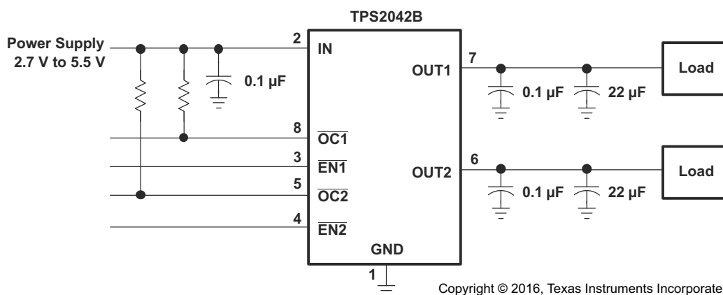
图 9-1. Typical Application (Example, TPS2042B)
