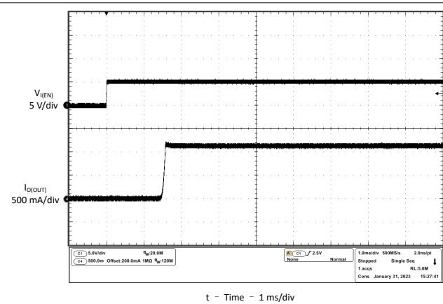
图 6-42. Short-Circuit Current, Device Enabled Into Short
