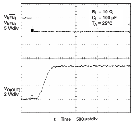
图 9-20. Turnon Delay and Rise Time With 100-μF Load
