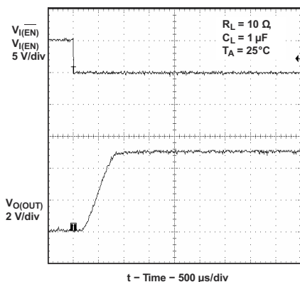
图 9-18. Turnon Delay and Rise Time With 1-μF Load
