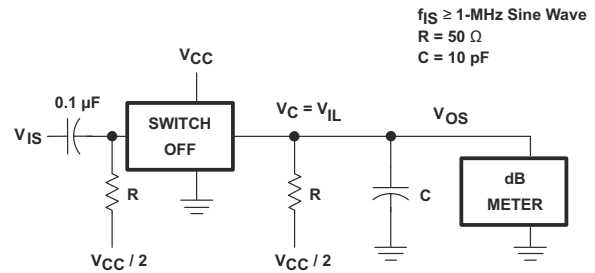
图 14-4. Switch OFF Signal Feedthrough Test Circuit
