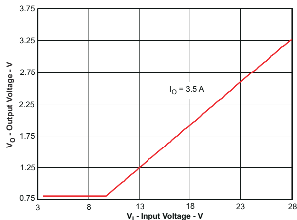
图 6-9. Typical Minimum Output Voltage vs Input Voltage
