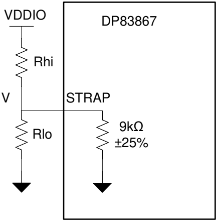
图 7-12. Strap Circuit
