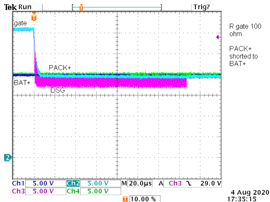
图 16-9. A Fast Turn-Off Case with a 100- \Omega Series Gate Resistor
