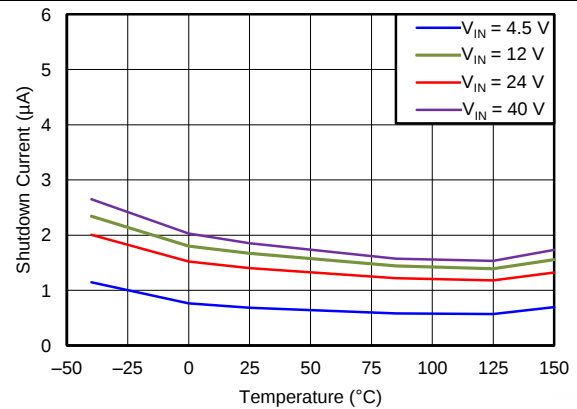
Figure 2. Shutdown Supply Current vs Temperature
