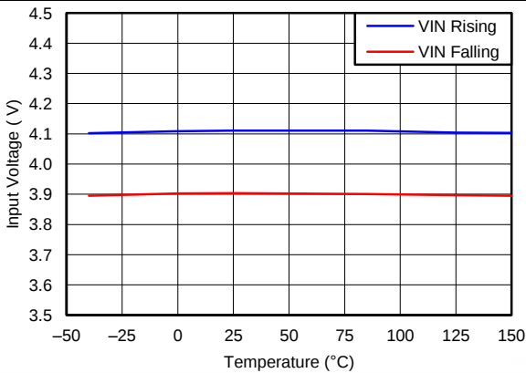
Figure 1. Input Start and Stop Voltage vs Temperature
