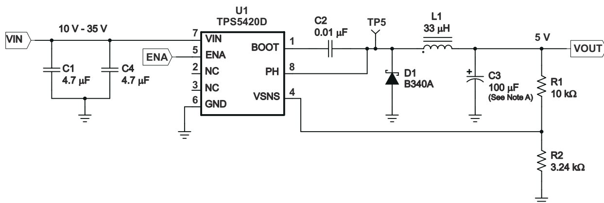
图 8-3. Application Circuit, 10-V — 35 V to 5-V
