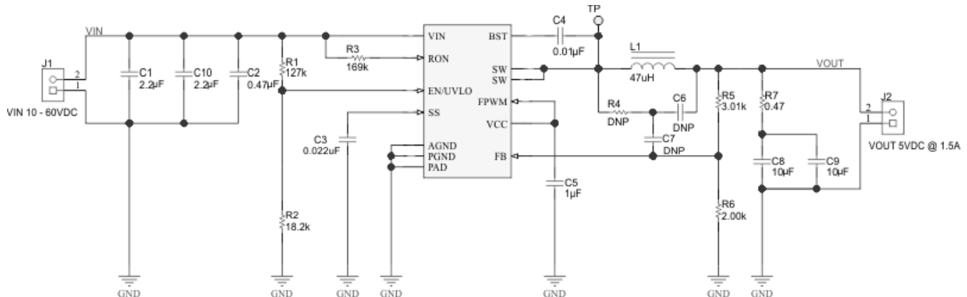
Figure 19. LM5160 Synchronous Buck Application Circuit
