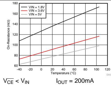
图 4. On-Resistance vs Junction Temperature
