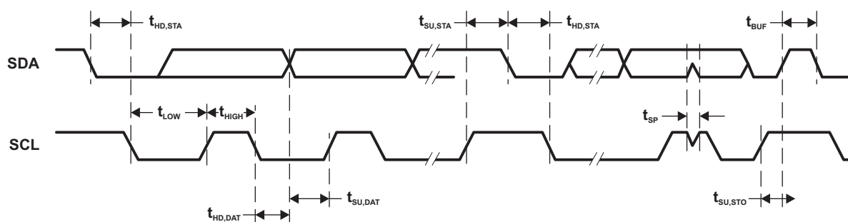
Figure 20. I2C 模式定时
