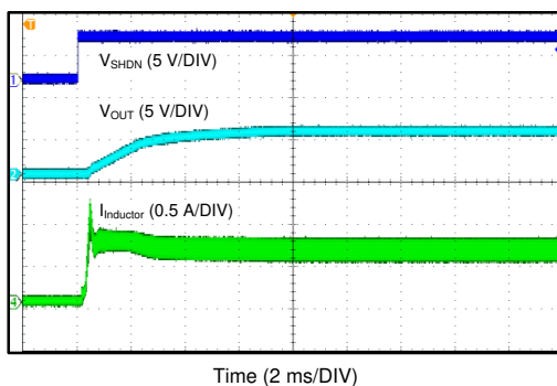
图 8-6. Start-up Waveform
