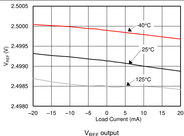
图 7-12. Output Voltage Change vs Load Current ( V_{REF} )
