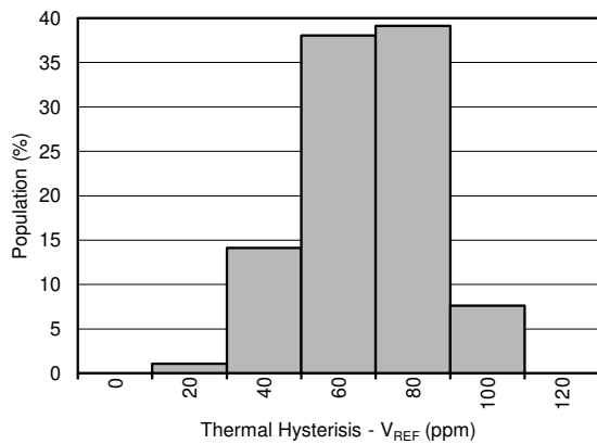
图 8-5. Thermal Hysteresis Distribution (V REF )
