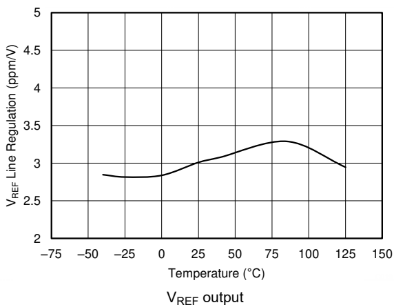
图 7-18. Line Regulation vs Temperature ( V_{REF} )
