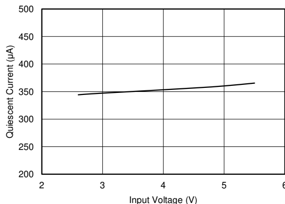
图 7-32. Quiescent Current vs Input Voltage
