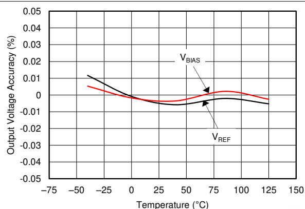
图 7-10. Output Voltage Accuracy ( V_{REF} ) vs Temperature
