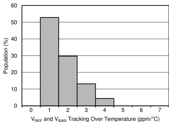
图 7-7. Distribution of V_{REF} - 2 \times V_{BIAS} Drift Tracking Over Temperature
