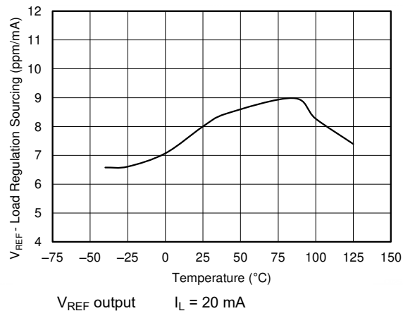
图 7-14. Load Regulation Sourcing vs Temperature ( V_{REF} )
