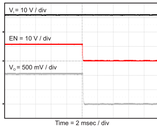
Figure 32. TPS562209 Shut Down Relative to EN
