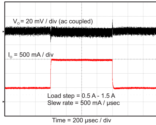
Figure 28. TPS562209 Transient Response
