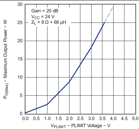
Gain = 20 dB V_{CC} = 24\text{ V} Z_L = 8\ \Omega + 66\ \mu\text{H}
