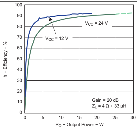
Gain = 20 dB Z_L = 4\ \Omega + 33\ \mu\text{H}
