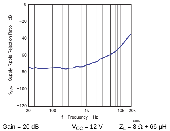
Figure 14. Supply Ripple Rejection Ratio vs Frequency
