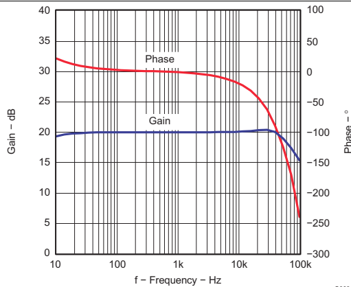
Gain = 20 dB V_{CC} = 12\text{ V} Z_L = 8\ \Omega + 66\ \mu\text{H} C_1 = \mu\text{F} V_I = 0.1\text{ V}_{\text{RMS}}
