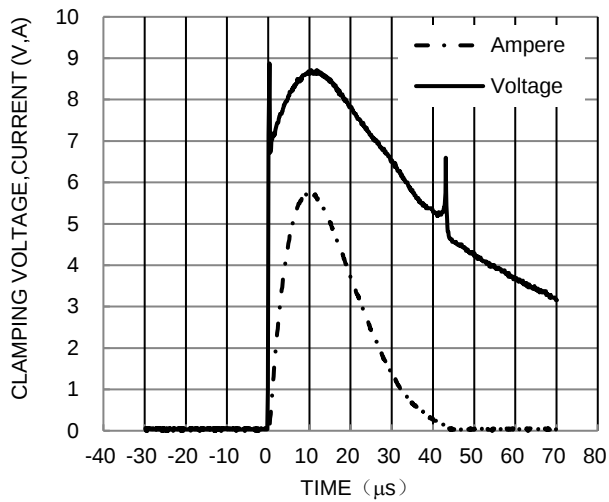
Figure 3. Waveform of Clamping Voltage, Current vs. Time (8/20μs, I/O to V_{SS} )
