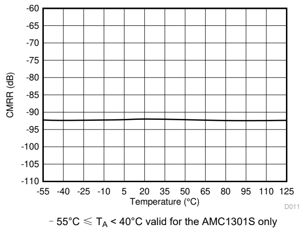
图 6-14. Common-Mode Rejection Ratio vs Temperature
