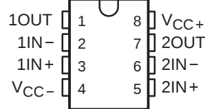
TLE2062, TLE2062A, TLE2062B D, JG, OR P PACKAGE (TOP VIEW)
