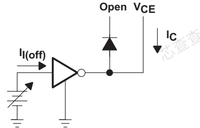
Figure 4. I_{I(off)} Test Circuit
