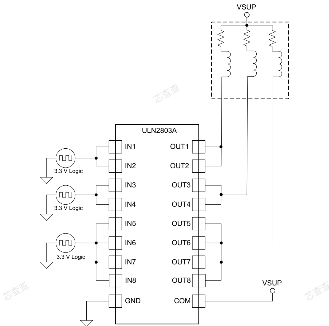
Figure 12. ULN2803A as Inductive Load Driver
