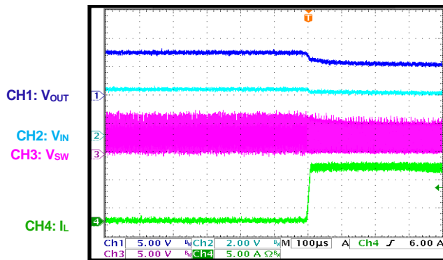
Over-Current Entry Increased output current, 0A to 4.5A
