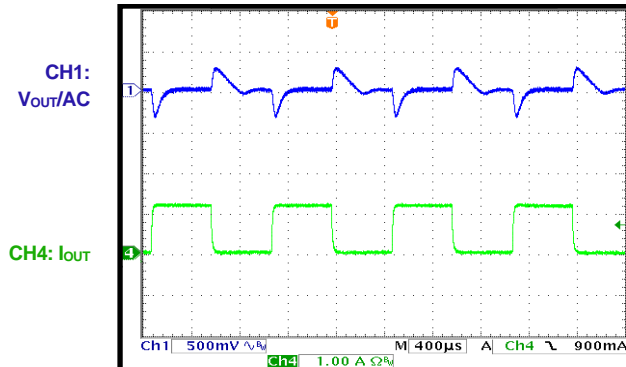
Load Transient I_{OUT} = 0A to 1.25A , USM
