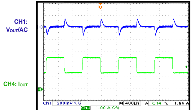
Load Transient I_{OUT} = 1.25A to 2.5A
