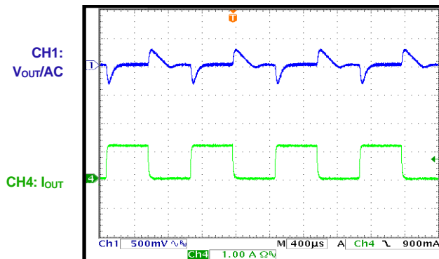
Load Transient I_{OUT} = 0A to 1.25A , PSM
