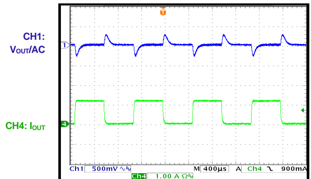
Load Transient I_{OUT} = 0A to 1.25A , FCCM
