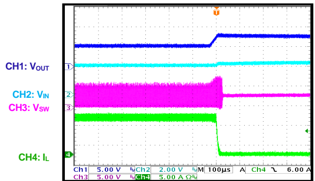
Over-Current Recovery Decreased output current, 4.5A to 0A
