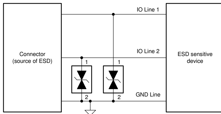
Application Schematic
