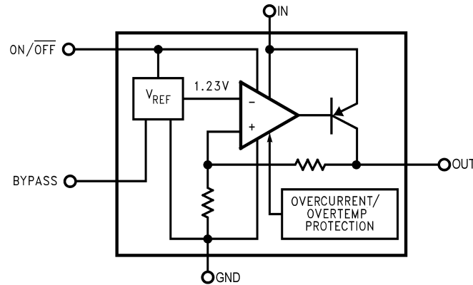
图 7-1. Block Diagram for Legacy Chip
