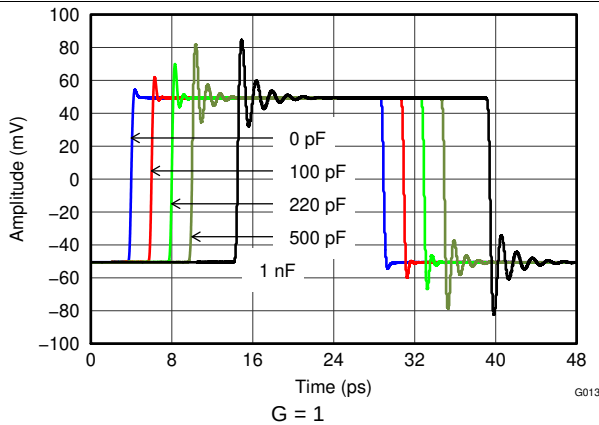
Figure 51. Small-Signal Response Over Capacitive Loads
