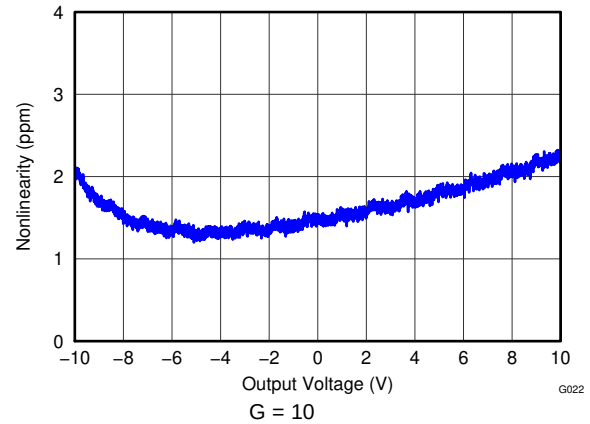
Figure 38. Gain Nonlinearity
