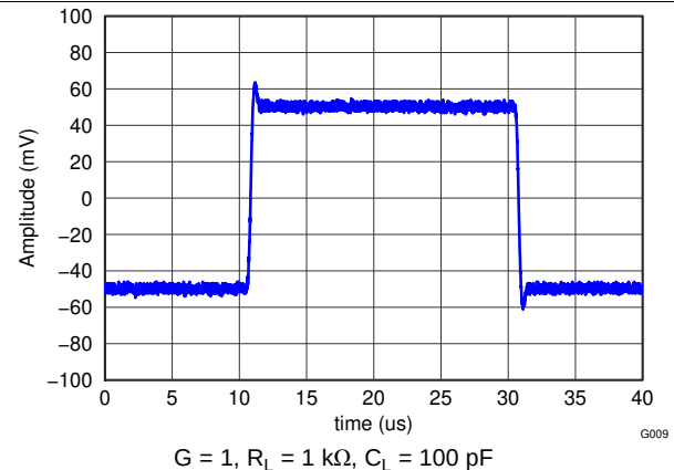
Figure 52. Small-Signal Response
