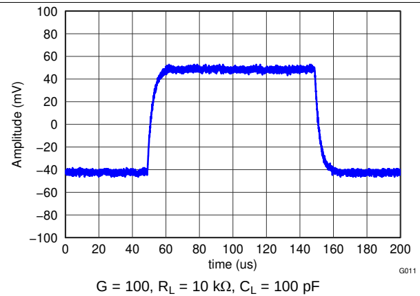
Figure 54. Small-Signal Response
