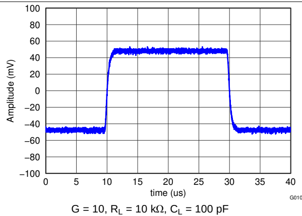
Figure 53. Small-Signal Response
