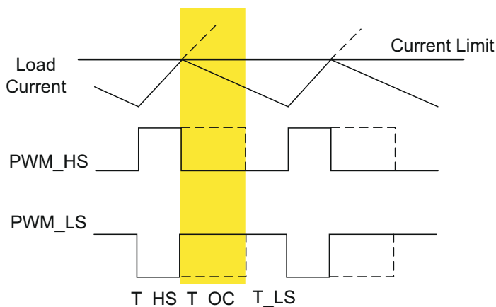
图 6-1. Cycle-by-Cycle Operation With High-Side OC
