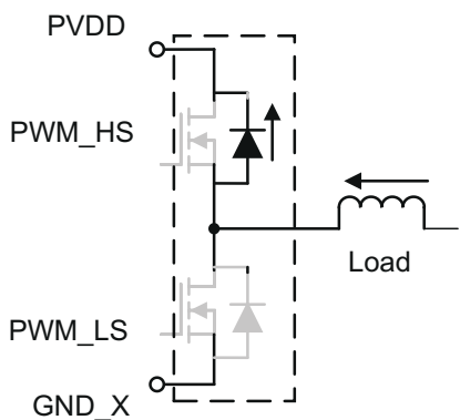
图 6-2. Cycle-by-Cycle Operation With Low-Side OC
