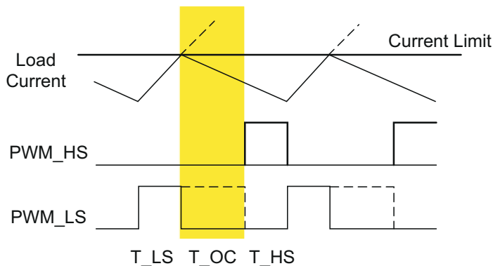
图 6-2. Cycle-by-Cycle Operation With Low-Side OC
