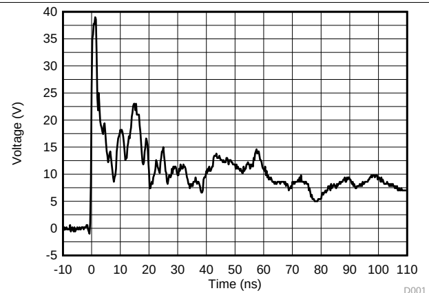
Figure 11. 8-kV IEC Waveform through 2m HDMI Cable
