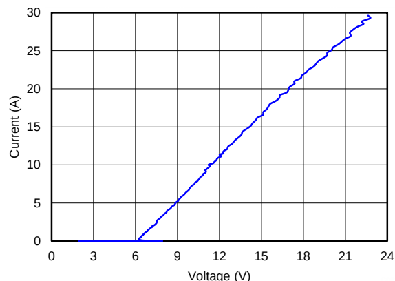
Figure 2. Negative TLP Curve
