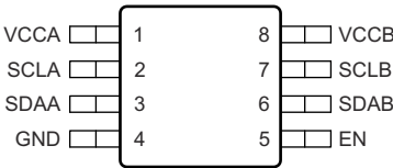
图 4-3. DGK Package, 8-Pin VSSOP Top View
