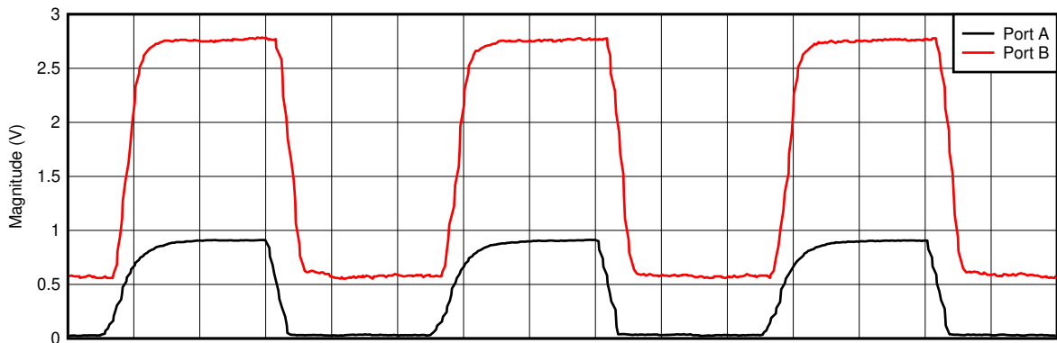
图 8-6. Voltage Translation at 400 kHz, V_{CCA} = 0.9\text{ V} , V_{CCB} = 2.7\text{ V}
