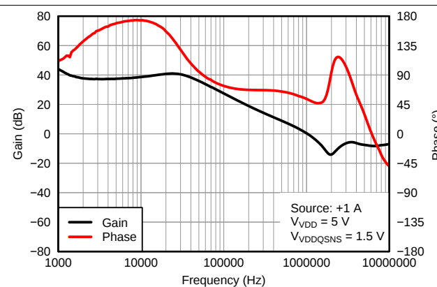
图 18. VTT (Source: +1 A) Bode Plot (0.75 V)
