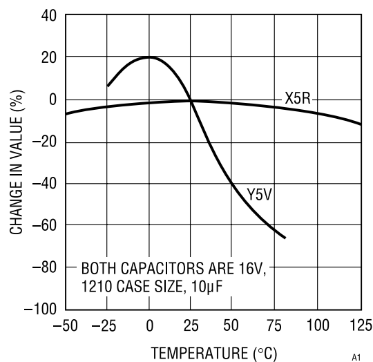
Figure17.b. Ceramic Capacitor DC Bias Characteris
