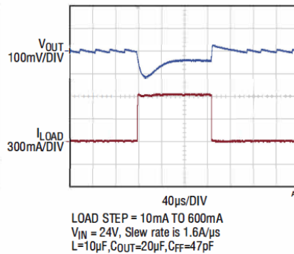
Load Transient, VOUT = 5V
