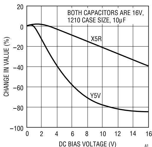
Figure17.a Ceramic Capacitor DC Bias Characteris
