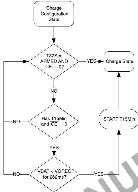
Figure 38. Charge Configuration
