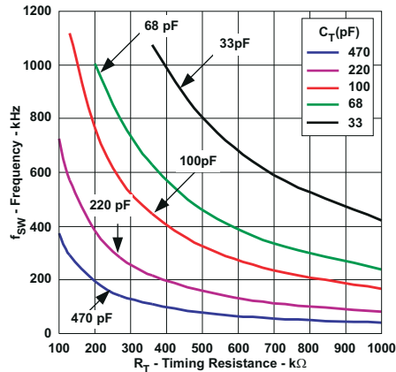
图 6-1. Frequency vs Timing Resistance
