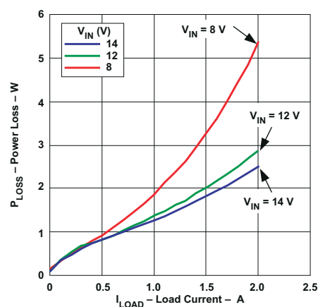
图 8-5. Power Loss vs Load Current
