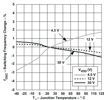
图 6-10. Switching Frequency Change vs Junction Temperature
