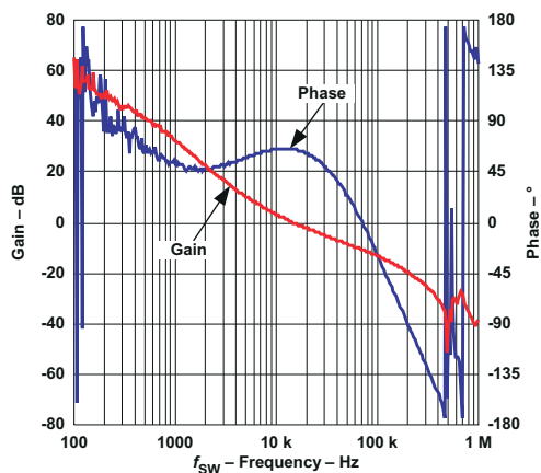
图 8-2. Gain and Phase vs Frequency
