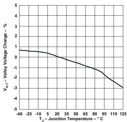
图 6-16. Valley Voltage Change vs Junction Temperature
