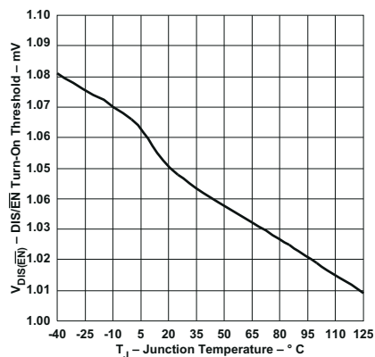
图 6-18. DIS/EN Turn-On Threshold vs Junction Temperature
