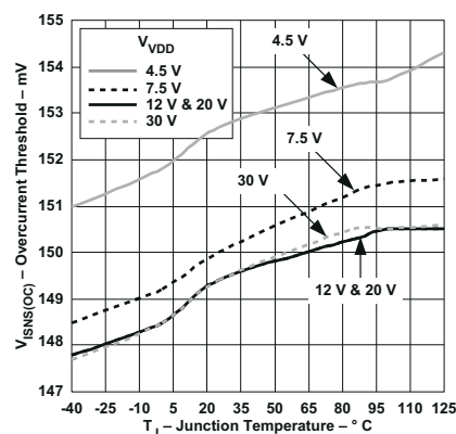
图 6-8. Overcurrent Threshold vs Junction Temperature
