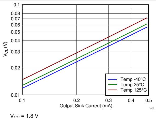
图 6-16. Output Voltage Low vs Output Sink Current
