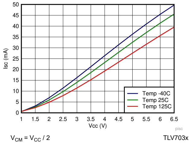
图 6-21. Output Short Circuit (Source) vs V_{CC}
