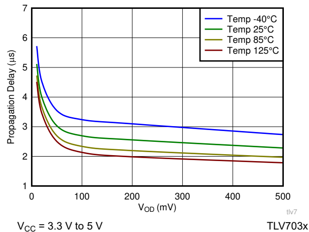
图 6-25. Propagation Delay (L-H) vs Input Overdrive
