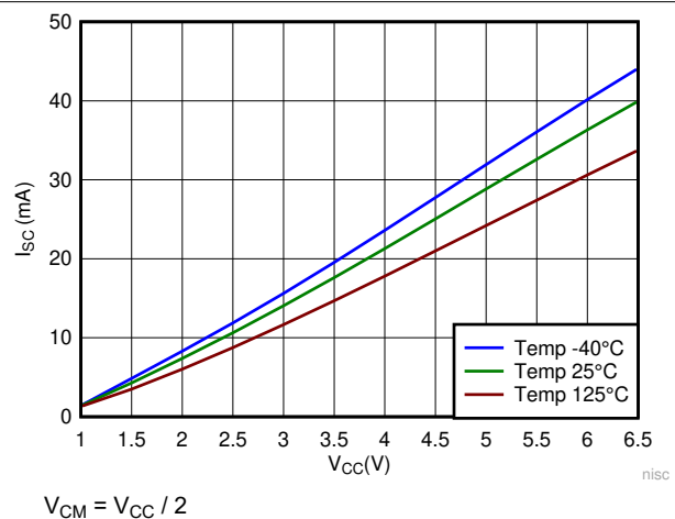
图 6-20. Output Short Circuit (Sink) vs V_{CC}
