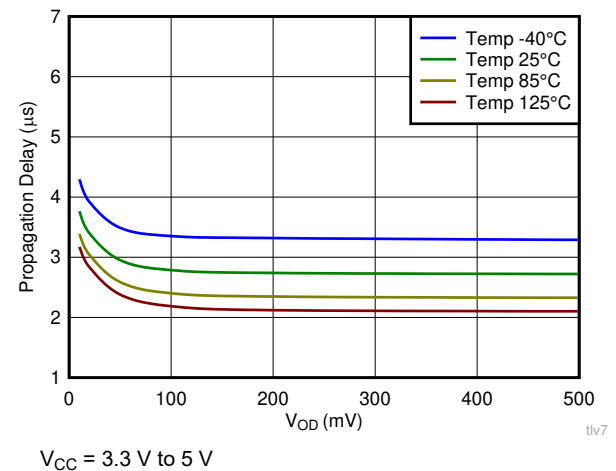
图 6-26. Propagation Delay (H-L) vs Input Overdrive
