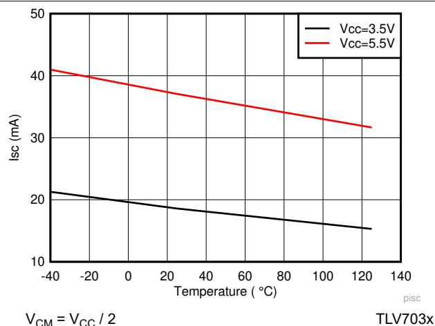
图 6-19. Output Short-Circuit (Source) Current vs Temperature
