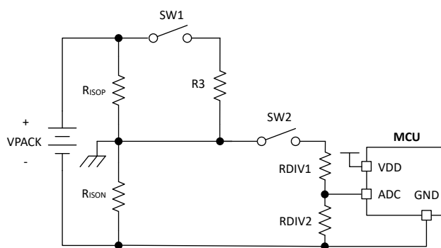
图 9-3. Battery V- Reference Architecture
