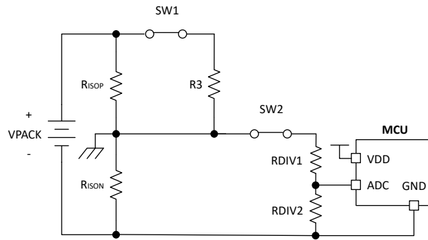
图 9-5. Battery V-Reference Switch Positions for ADC2 Measurement
