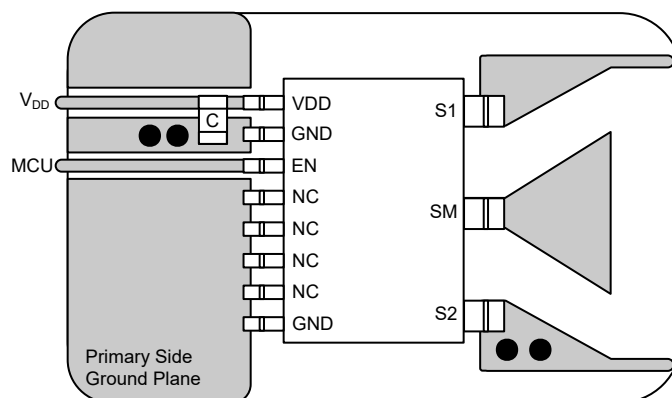
图 9-21. TPSI2140-Q1 Layout with Interlayer Stitch Capacitance: Top Layer (1)
