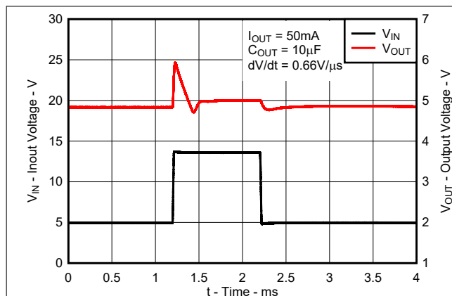
图 8-10. Dropout Exit Transient Response for New Chip
