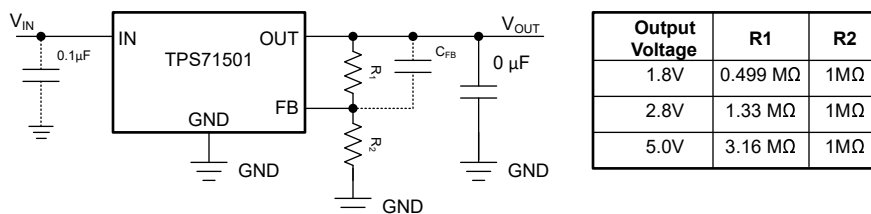
图 8-2. TPS71501 Adjustable LDO Regulator Programming
