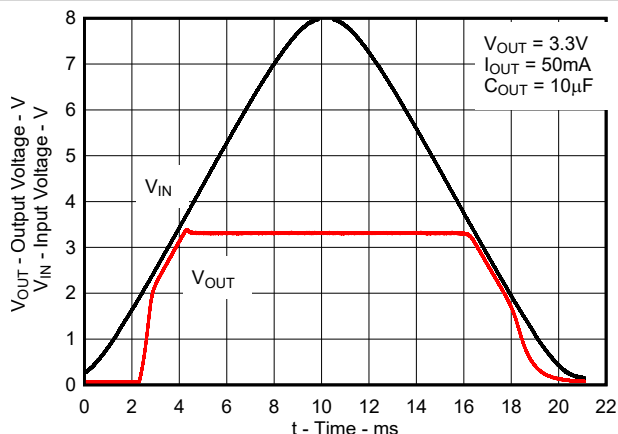
图 8-5. Power-Up and Power-Down for New Chip
