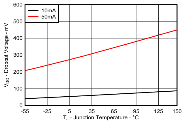
图 6-14. Dropout Voltage vs Junction Temperature for New Chip
