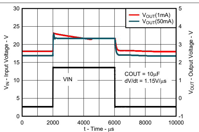
图 8-11. Fast Line Transient Response for New Chip
