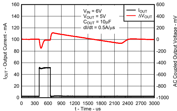
图 8-9. Load Transient Response for New Chip
