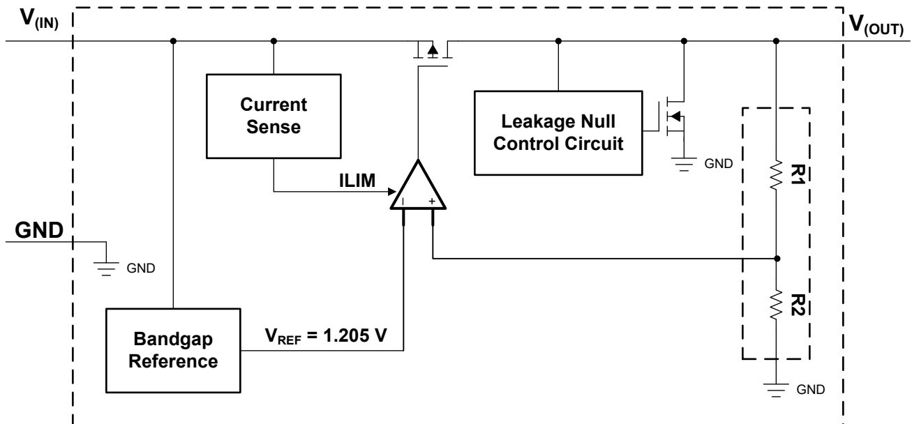
图 7-2. Functional Block Diagram—Fixed Version
