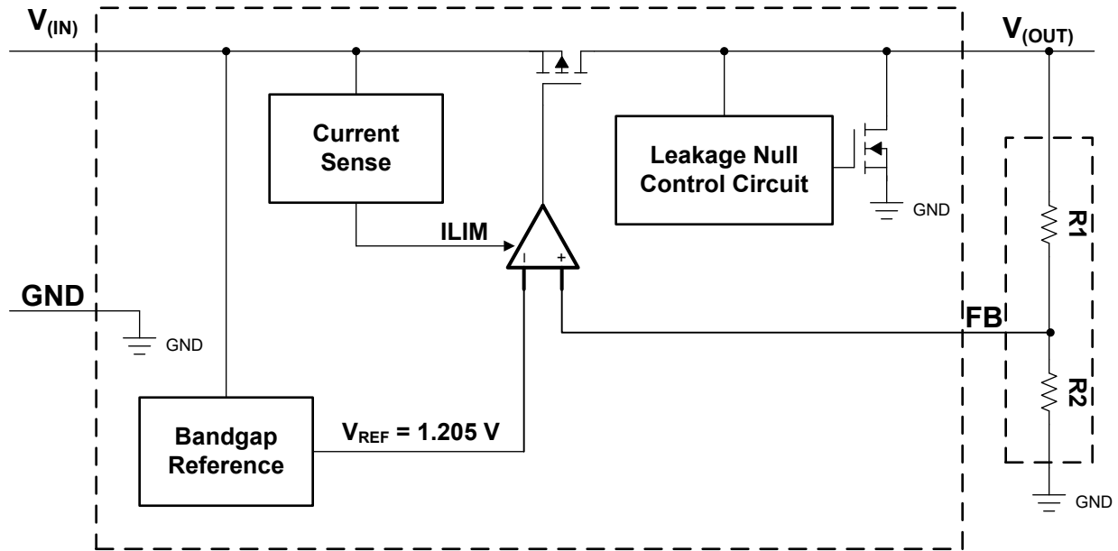
图 7-1. Functional Block Diagram—Adjustable Version
