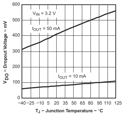
图 6-13. Dropout Voltage vs Junction Temperature for Legacy Chip
