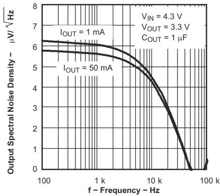
图 6-7. Output Voltage Spectral Noise Density vs Frequency for Legacy Chip
