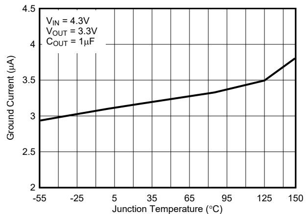
图 6-6. Quiescent Current vs Junction Temperature for New Chip
