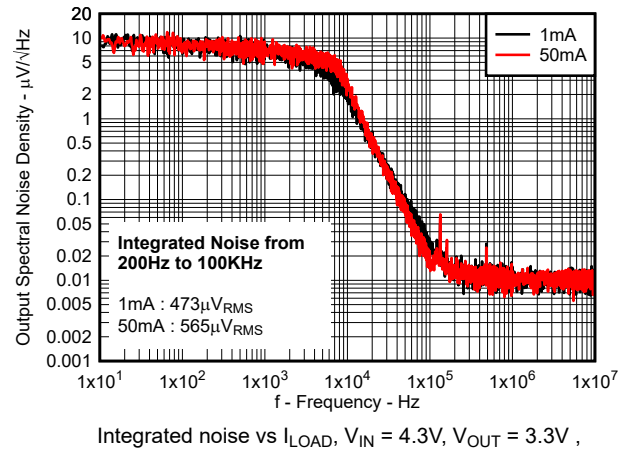
图 6-8. Output Voltage Spectral Noise Density vs Frequency for New Chip
