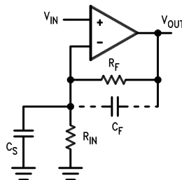
图 6-2. General Operational Amplifier Circuit
