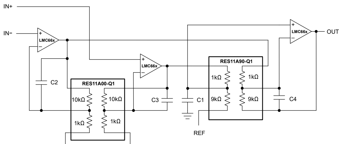
图 6-8. Improved Instrumentation Amplifier With the RES11A
