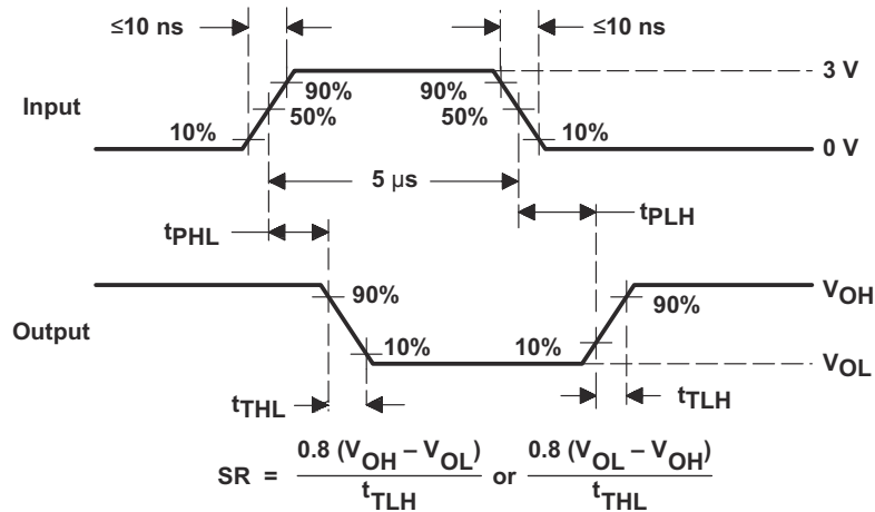
WAVEFORMS
