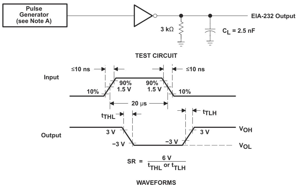
图 6-2. Driver Test Circuit and Waveforms for t_{PHL} and t_{PLH} Measurements ( 5\ \mu s Input)
