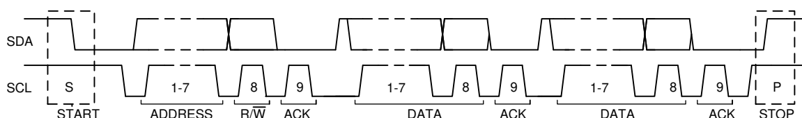
图 9-19. Complete Data Transfer on the I²C Bus
