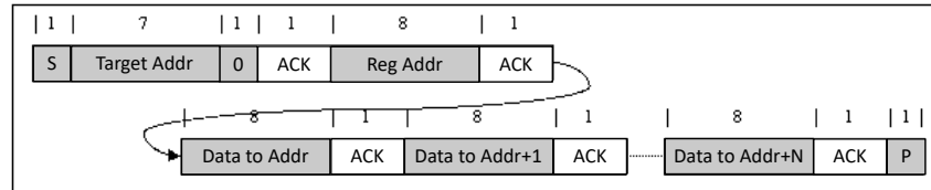
图 9-22. Multi-Write
