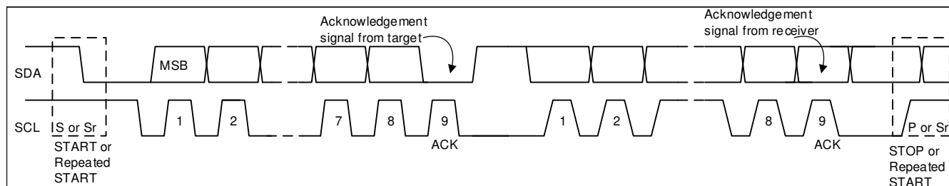
图 9-17. Data Transfer on the I²C Bus
