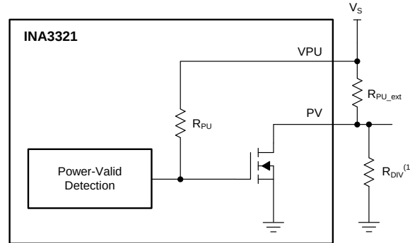
图 20. Power-Valid Output Structure
