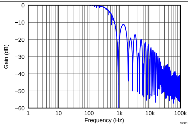
图 1. Frequency Response
