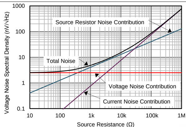
图 8. Voltage Noise vs Source Resistance
