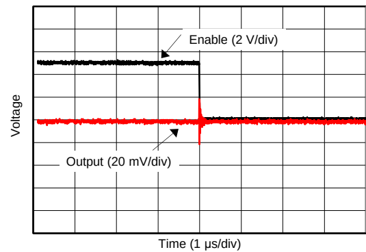
图 47. OPA1622 Output Voltage When Enable Pin Transitions Low (32- \Omega Load Connected)
