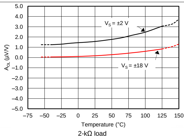
图 12. Open-Loop Gain vs Temperature
