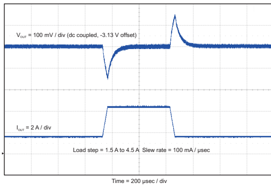
Figure 32. Load Transient
