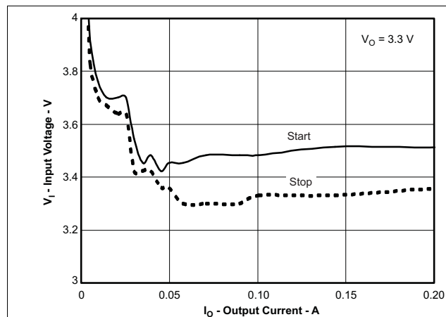
Figure 25. 3.3-V Start/Stop Voltage
