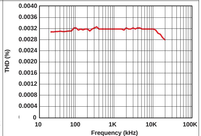
Figure 17. Total Harmonic Distortion vs Frequency ( R_L = 600 \Omega )
