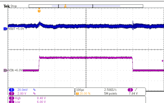
图 10-57. Line Transient Response
