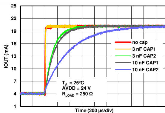
图 8-7. IOUT vs Time for Different Capacitor Values on CAP1 and CAP2
