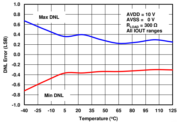
图 7-63. IOU DNL vs Temperature (Internal R_{SET} )
