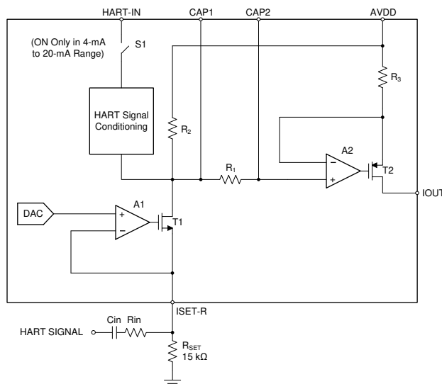
图 9-4. Implementing HART With the ISET-R pin
