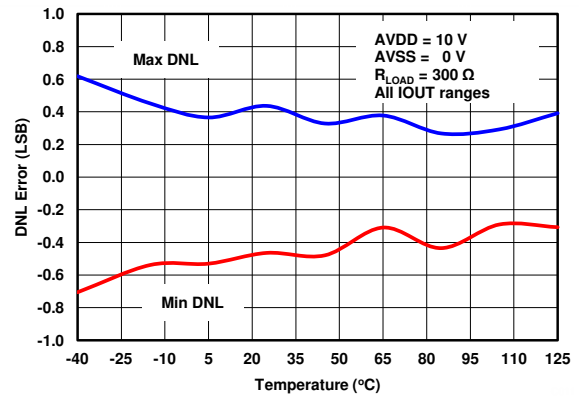
图 7-64. IOU DNL vs Temperature (External R_{SET} )
