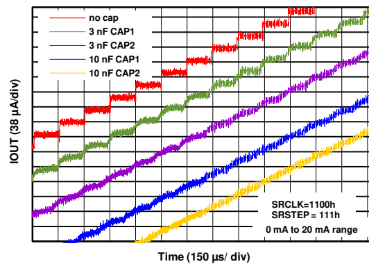
图 8-5. IOUT vs Time With Digital Slew Rate Control
