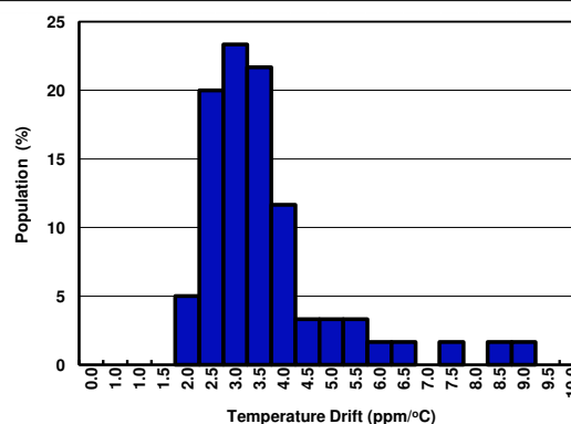
图 7-4. Internal Reference Temperature Drift Histogram
