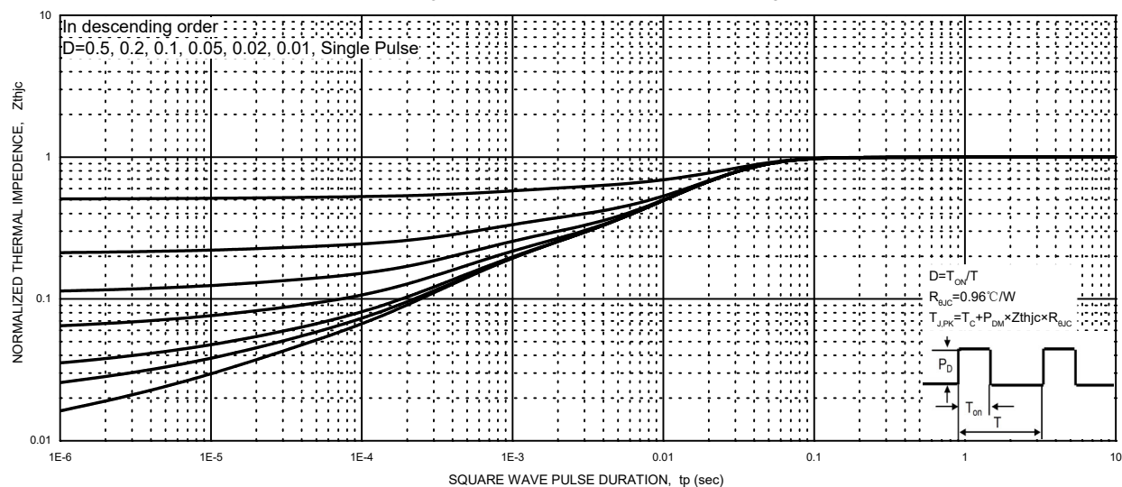
NORMALIZED TRAISIENT THERMAL IMPENDANCE
