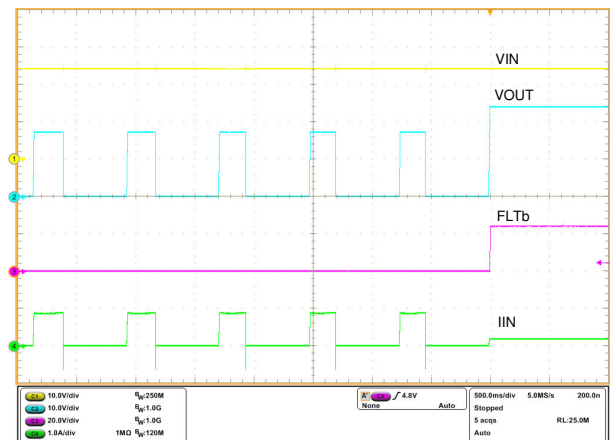
Load transition from 20 Ω to 120 Ω VIN = 24 V, R LIM = 7.5 kΩ
