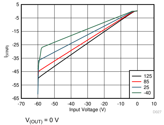
图 7-10. Input Supply Current vs Reverse Supply Voltage, -V_{(IN)}
