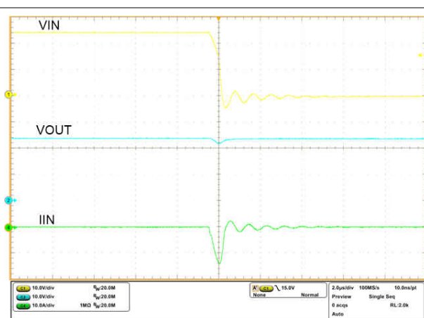
图 9-14. Hot-Short: Fast-Trip Response (Zoomed)
