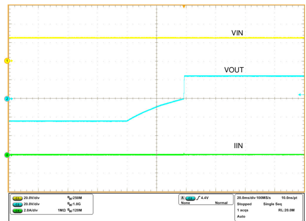
图 9-7. Response During Coming Out of Output Reverse Polarity Fault Condition
