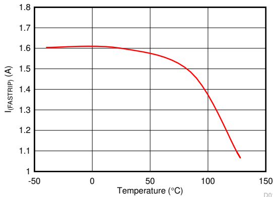
图 7-19. Fast-Trip Comparator Threshold I_{\text{FAST-TRIP}} vs Temperature Threshold
