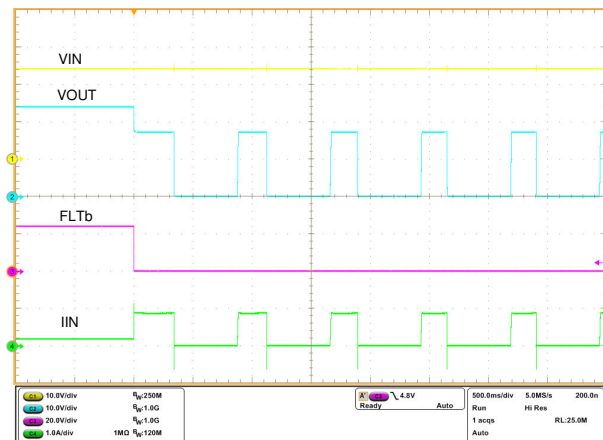
Load transition from 120 Ω to 20 Ω VIN = 24 V, R LIM = 7.5 kΩ
