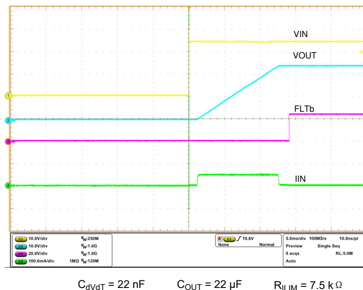
图 9-3. Hot Plug-In and Inrush Current Control at 24-V Input
